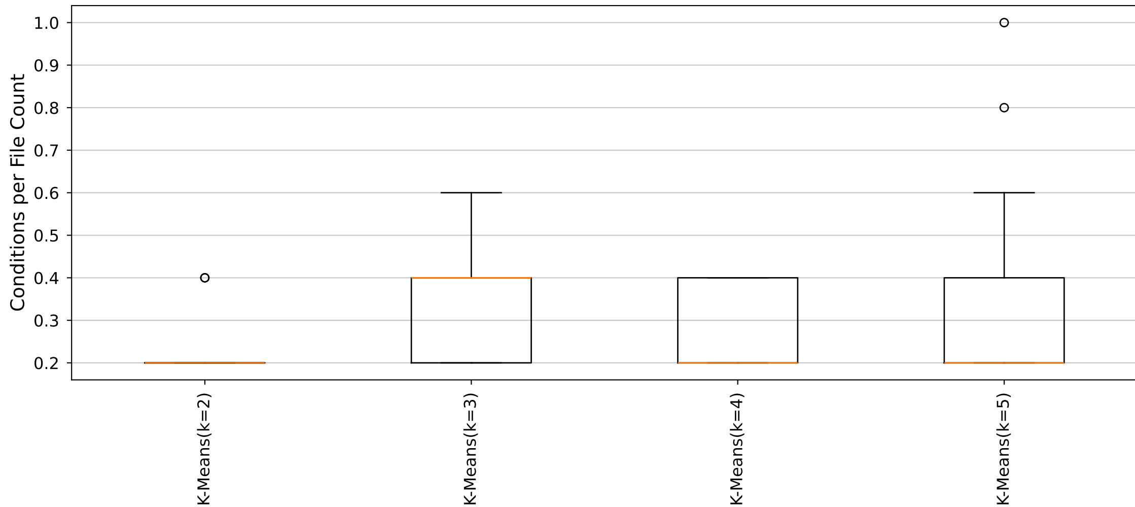
YARA Rules Conditions per File Count Distribution (Cluster34_Size5 dataset)
